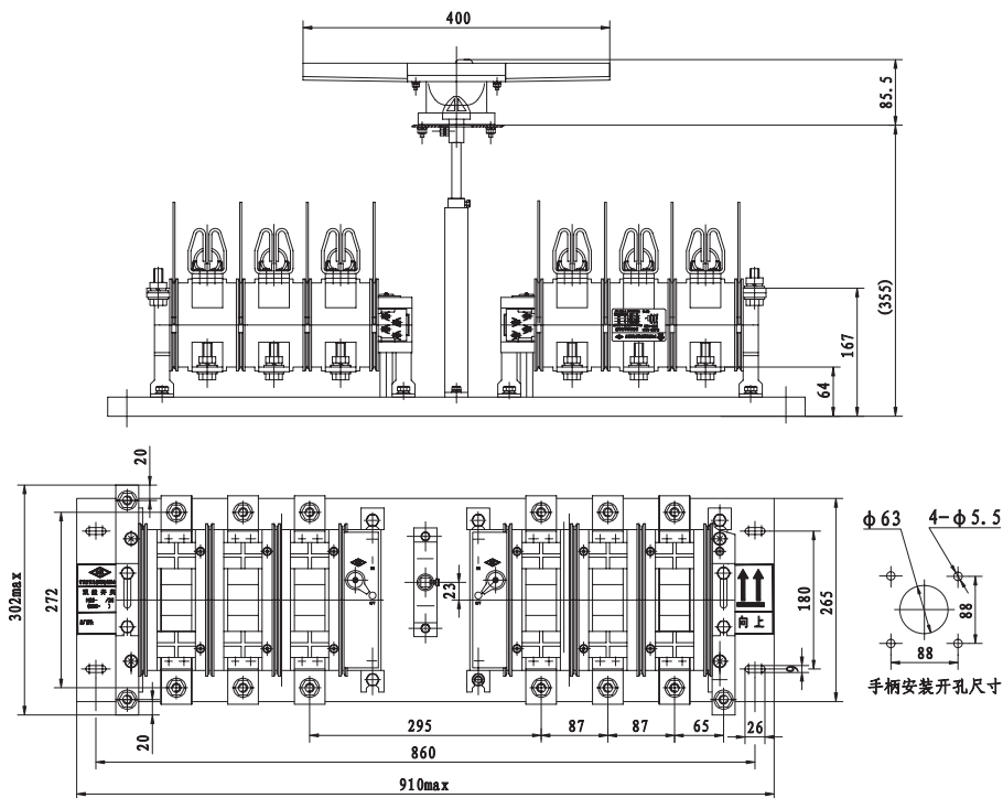
HSS-630、800/3N
